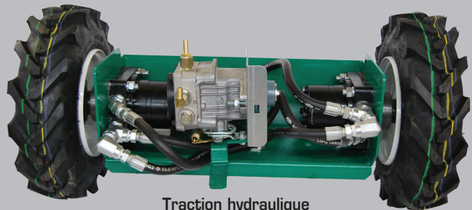
Traction hydraulique
